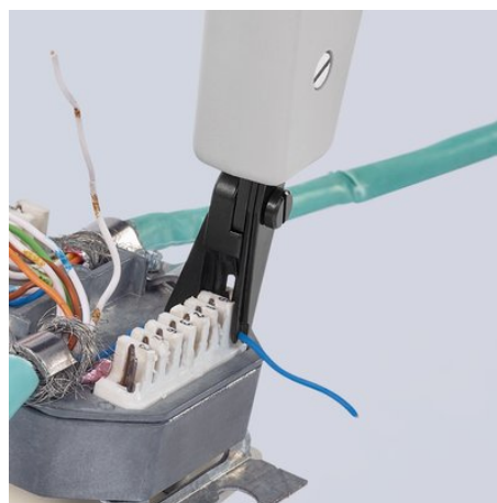
Inserts and cuts cables in one operation
