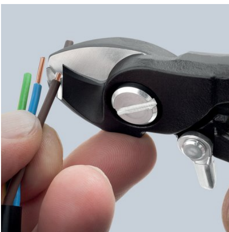
95 41 165: with stripping function
