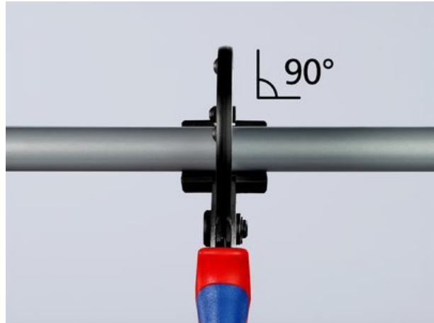
The wide plastic supports opposite the cutting wheel allow perfect right-angled cuts
