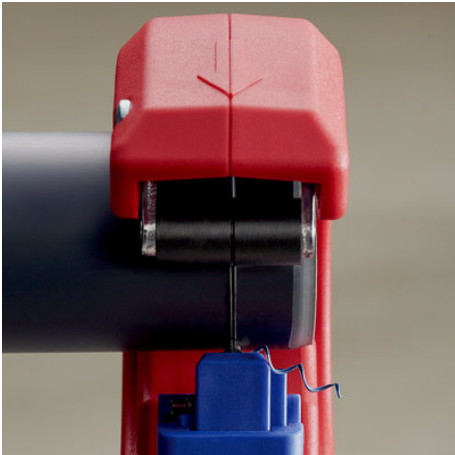
Segments as short as 10 mm can be cut. The spiral chip comes from chamfering.
