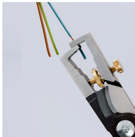
Length mark: Profiling on the inner side helps when stripping wire in standard lengths (11 mm and 16 mm)
