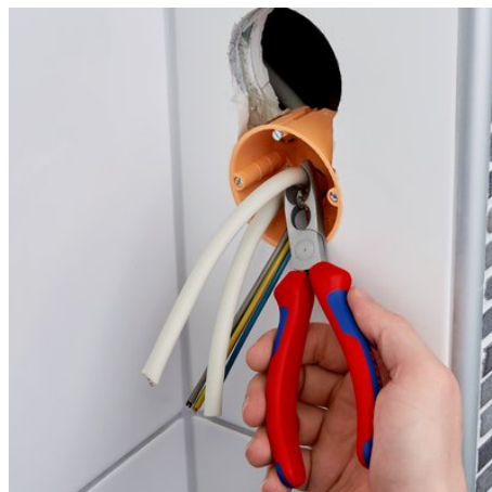
Stripping deep down in a flush-mounted junction box
