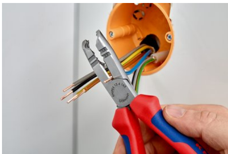
Cutting when shortening single conductors
